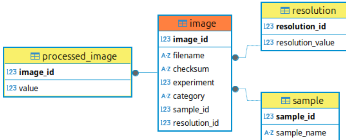
Fig. 8.1: The ERD of the AdvProcessor.
